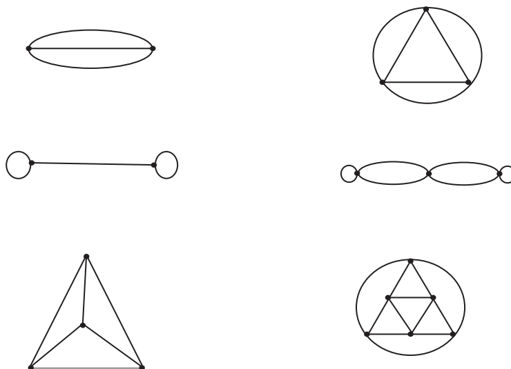
FIGURE 3.1. Examples of cell graphs (left) and corresponding \Gamma_0 graphs (right). Top: the double SG. Note that the three vertices of \Gamma_0 form two distinct triangles. Middle: Note that \Gamma_0 has two degenerate triangles with just two vertices. Bottom: the octahedron fractafold.
